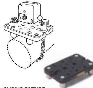
SLIDING FIXTURE Used when the shafts cannot be rotated. Part Nr: 12-0039
