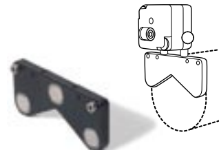
MAGNETIC FIXTURES Fixture for axial mounting on flange or shaft. Part Nr: 12-0038
